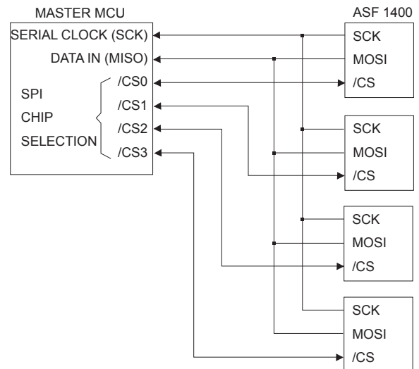
Figure 8: Cascading four ASF1400 devices using the SPI interface.
