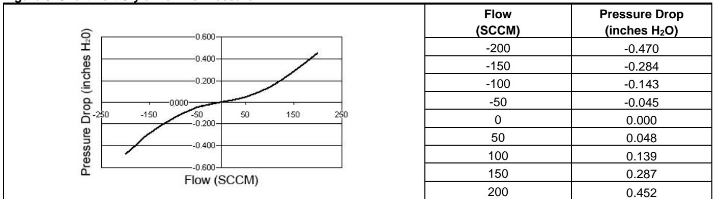
Figure 6. Short Port Style Flow vs Pressure
