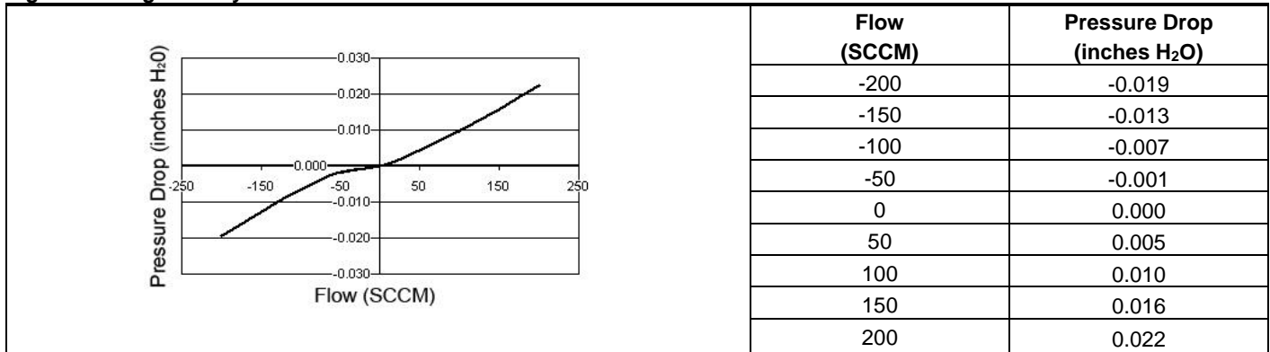
Figure 5. Long Port Style Flow vs Pressure
