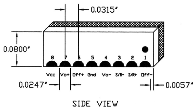
PACKAGE DRAWING HMC1051 ZL (8-PIN IN-LINE LCC)
