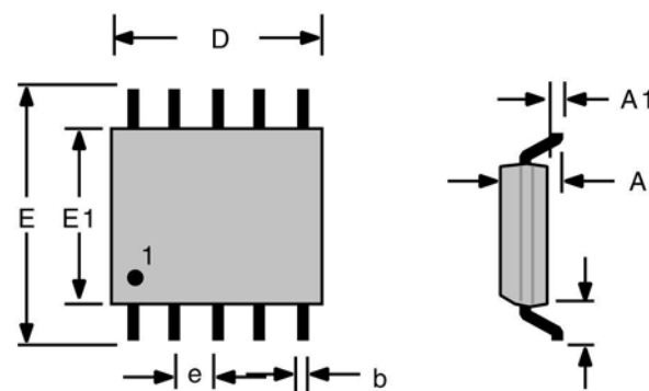
PACKAGE DRAWING HMC1052 (10-PIN MSOP)
