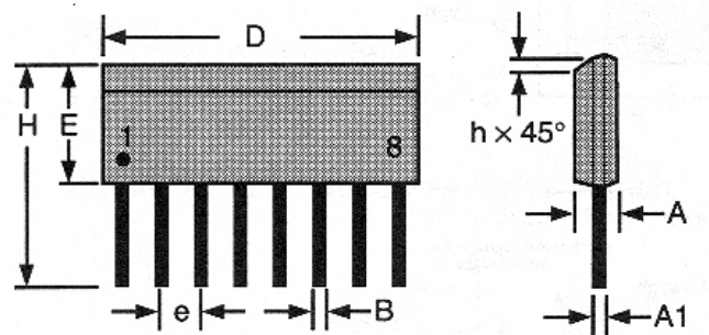
PACKAGE DRAWING HMC1051Z (8-PIN SIP)
